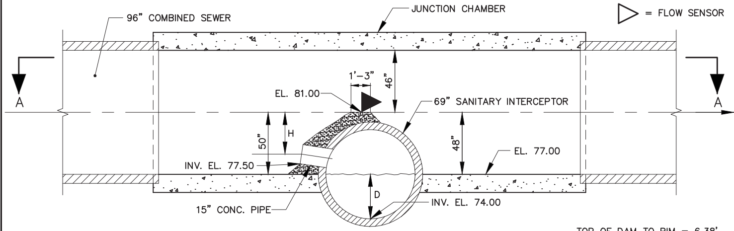
SECTION B-B
