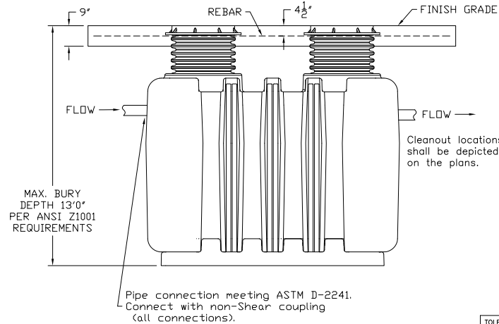
CONCRETE SLAB DETAIL FOR H2O/HS20 LOAD RATING
